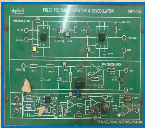
PULSE POSITION MODULATION & DEMODULATION
