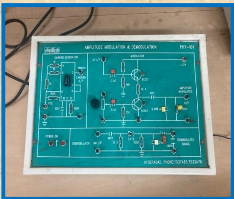
AMPLITUDE MODULATION & DEMODULATION
