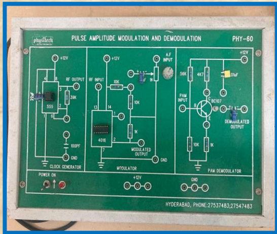
PULSE AMPLITUDE MODULATION & DEMODULATION TRAINER KIT
